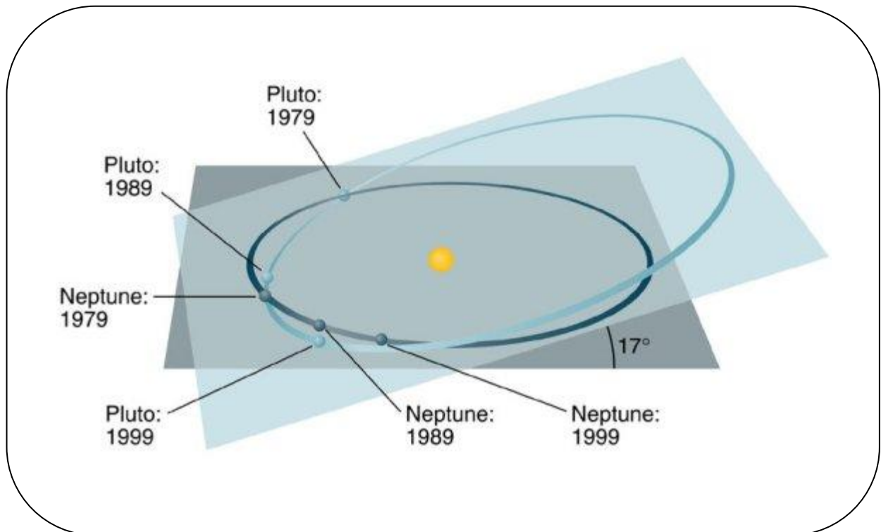
Comparison between the orbits of Pluto and Neptune
